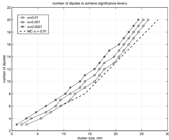
Fig. B.1. Number of dipoles required to achieve a given significance level \alpha as a function of cluster size for a fixed brain volume. The values are computed for total of N_d = 1000 dipoles using the approximate formula (B.3) for \alpha = 0.01, 0.001 and 0.0001 and using the Monte Carlo method for \alpha = 0.01 .
