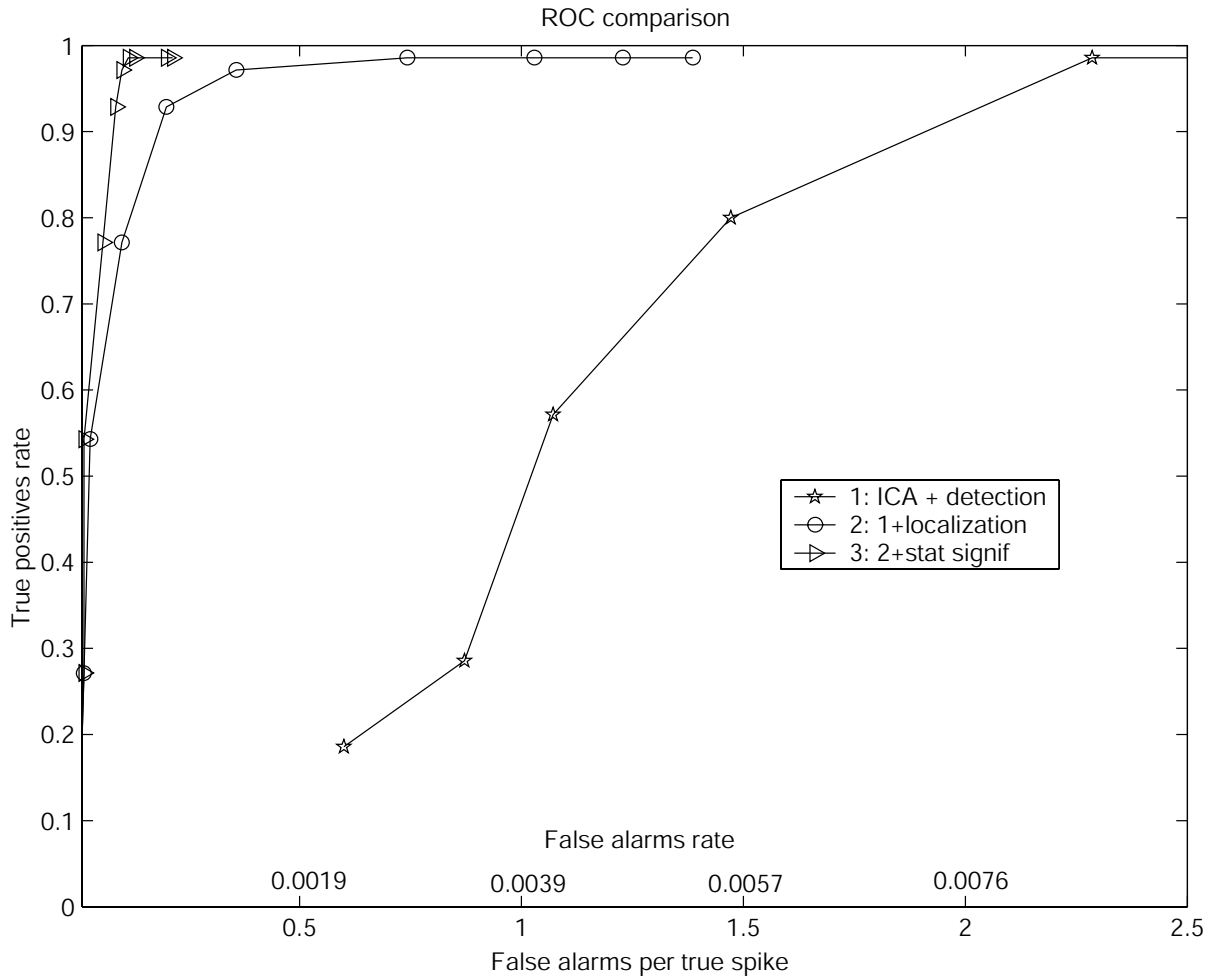
Fig. 3. Receiver Operating Characteristic (ROC) curves showing performance at three stages in the detection algorithm. Plotted for each stage of the processing are the true positive rate vs. false positive rate as described in the text. The results show clear improvement in sensitivity vs. specificity performance from Stage 1 to 2 and from Stage 2 to 3.
