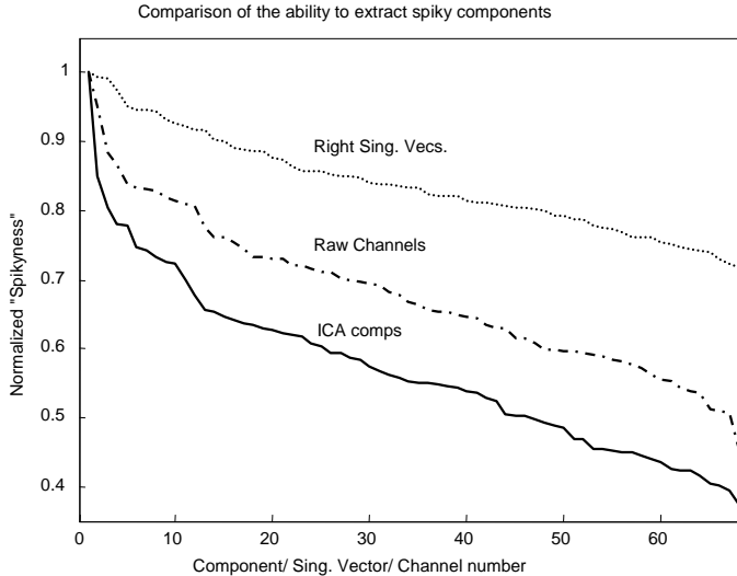
Fig. 1. Normalized "spikyness" spectrum for interictal MEG data computed from raw data and its decompositions using ICA and SVD. A decomposition that separates components containing spikes from those that do not will tend to exhibit a faster decrease in spikyness than the raw data; we refer to this characteristic as an increased degree of spikyness. Note that ICA increases the degree of spikyness compared to raw data while SVD actually reduces it.
