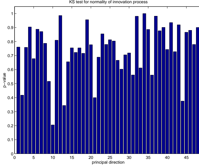
Fig. A.2. Computed p-values for Kolmogorov-Smirnov test for normality applied to residual or prediction errors using cross-validation data. The results indicate that there is no evidence in this data to support use of a distribution other than Gaussian to drive the MAR models.
