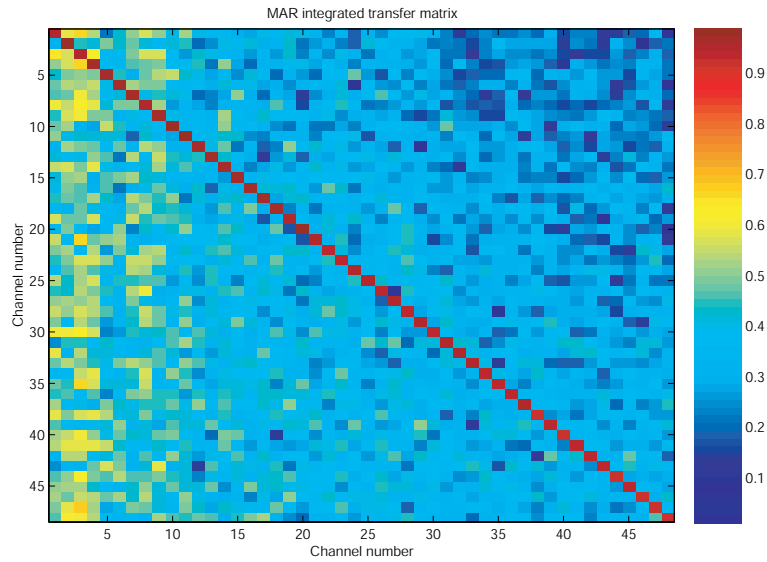
Fig. A.1. a) Prediction Error variance vs. MAR model order for estimated parameters when applied to cross-validation data. Note that the cross validation prediction error indicates a distinct minimum at model order P=4 ; b) The Integrated Directed Transfer Matrix for the estimated 4th order MAR parameters; the figure shows a high degree of correlation between channels in the data.
