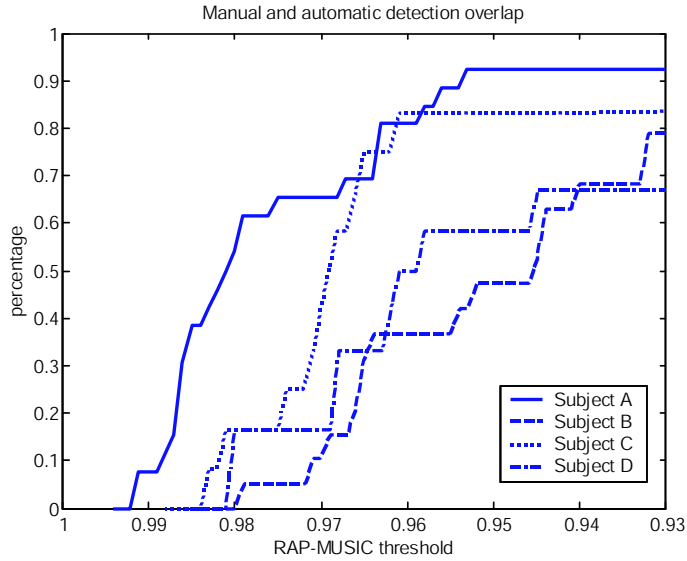
Fig. 9. Comparison of manual and automatic spike detection procedures. For each of the 4 subjects, we plot the fraction of the manually detected dipolar sources that are also found by the automated procedure. Different points on the curve are found using different acceptance thresholds during RAP MUSIC dipole localization. For the 4 subjects the following number of dipoles were found by the qualified reader: A: 13, B: 26, C: 12, D: 12
